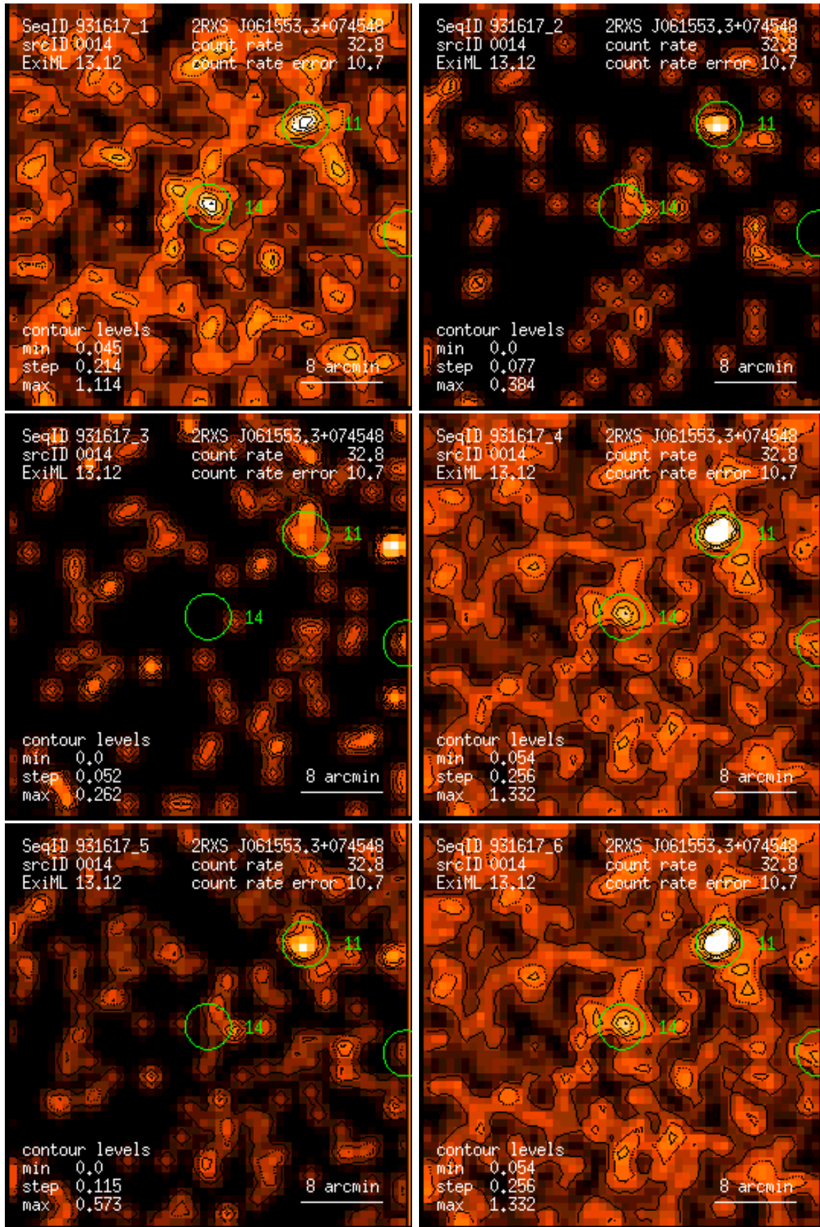
Figure 14: RASS 931617: detection 0014: band rate images, Gaussian filter: (1) PSPC channels 11 – 41, (2) 52 – 90, (3) 91 – 201, (4) 11 – 235, (5) 52 – 201, (6) 11 – 201. Broad band rates in counts/ks. Band rate contour levels in counts/ks/arcmin 2 .
