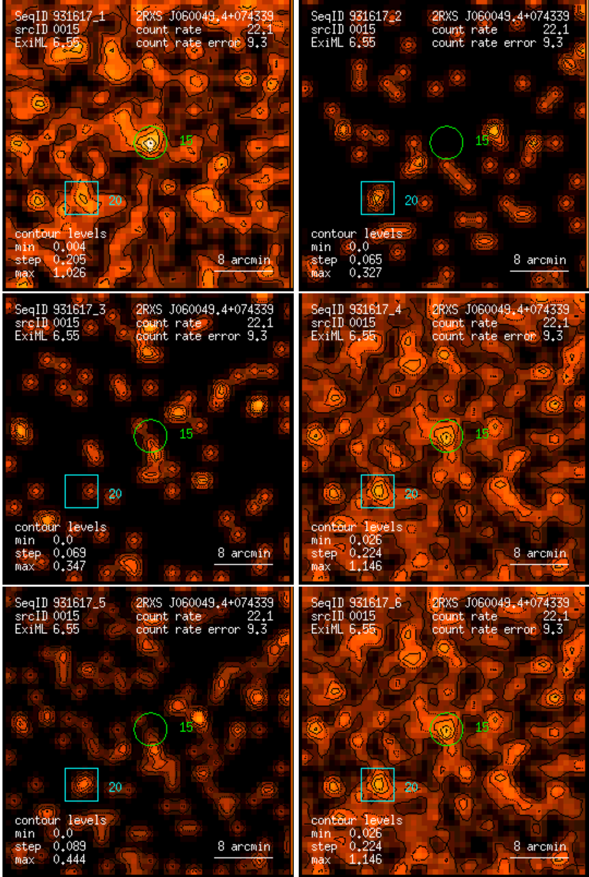
Figure 15: RASS 931617: detection 0015: band rate images, Gaussian filter: (1) PSPC channels 11 – 41, (2) 52 – 90, (3) 91 – 201, (4) 11 – 235, (5) 52 – 201, (6) 11 – 201. Broad band rates in counts/ks. Band rate contour levels in counts/ks/arcmin 2 .
