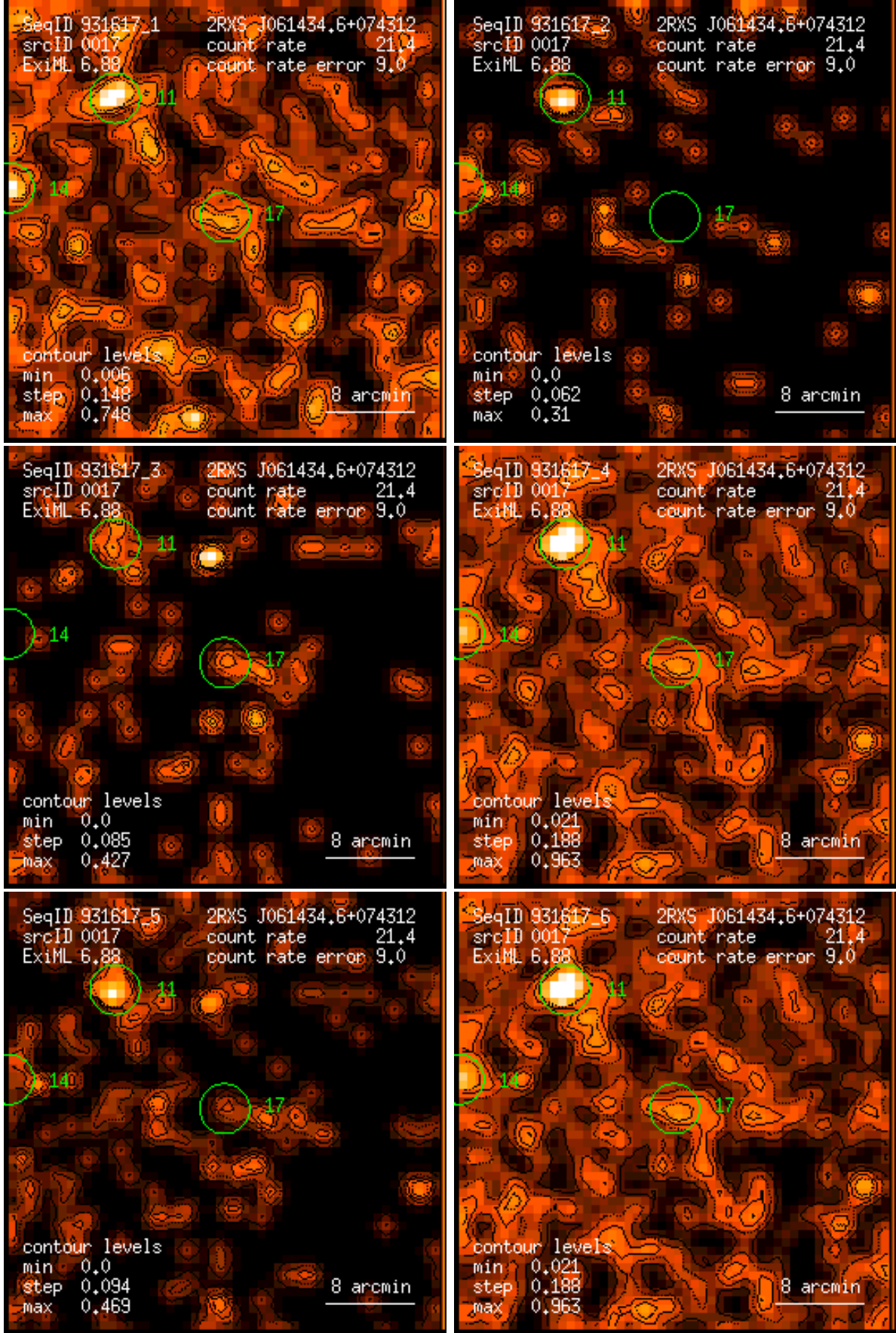
Figure 17: RASS 931617: detection 0017: band rate images, Gaussian filter: (1) PSPC channels 11 – 41, (2) 52 – 90, (3) 91 – 201, (4) 11 – 235, (5) 52 – 201, (6) 11 – 201. Broad band rates in counts/ks. Band rate contour levels in counts/ks/arcmin 2 .
