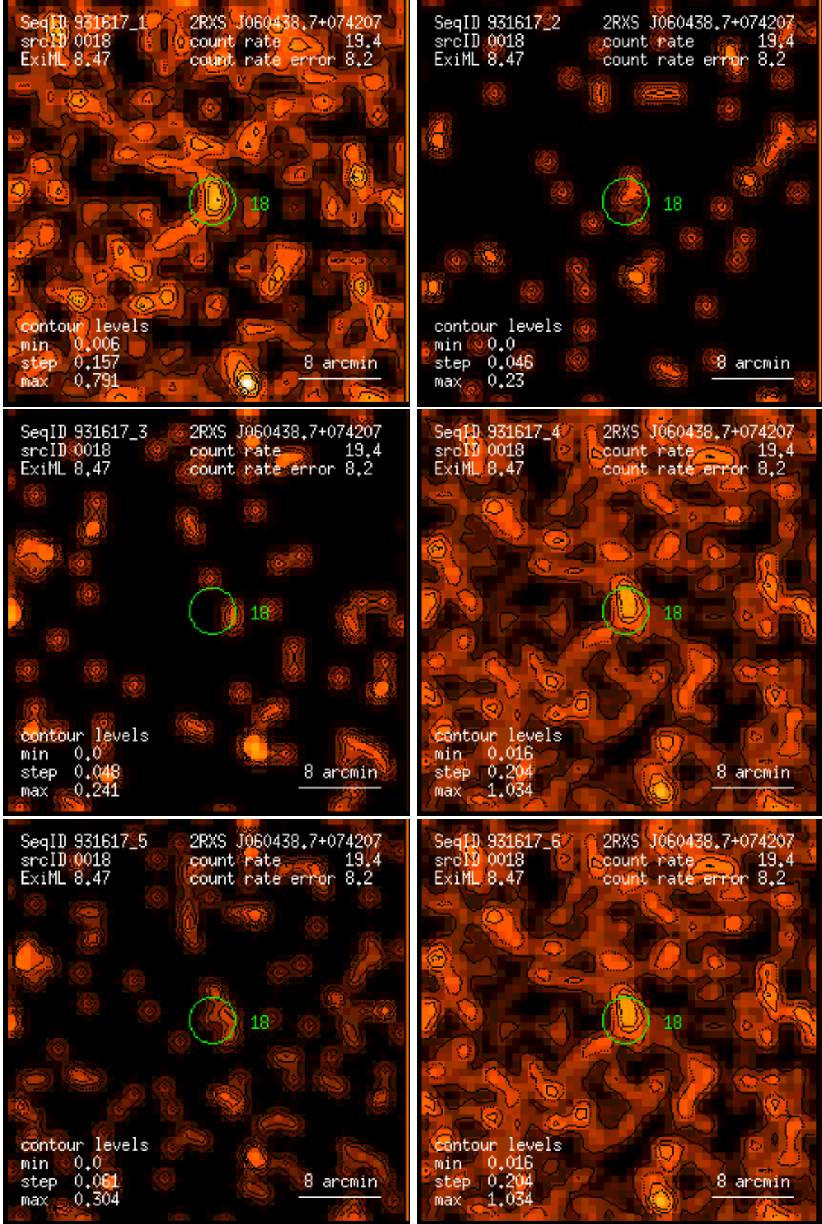
Figure 18: RASS 931617: detection 0018: band rate images, Gaussian filter: (1) PSPC channels 11 – 41, (2) 52 – 90, (3) 91 – 201, (4) 11 – 235, (5) 52 – 201, (6) 11 – 201. Broad band rates in counts/ks. Band rate contour levels in counts/ks/arcmin 2 .
