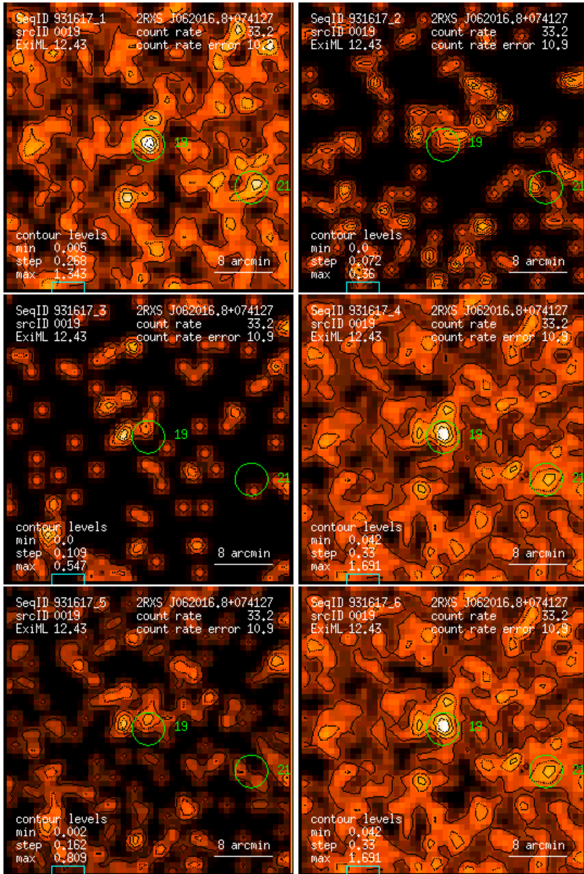
Figure 19: RASS 931617: detection 0019: band rate images, Gaussian filter: (1) PSPC channels 11 – 41, (2) 52 – 90, (3) 91 – 201, (4) 11 – 235, (5) 52 – 201, (6) 11 – 201. Broad band rates in counts/ks. Band rate contour levels in counts/ks/arcmin 2 .
