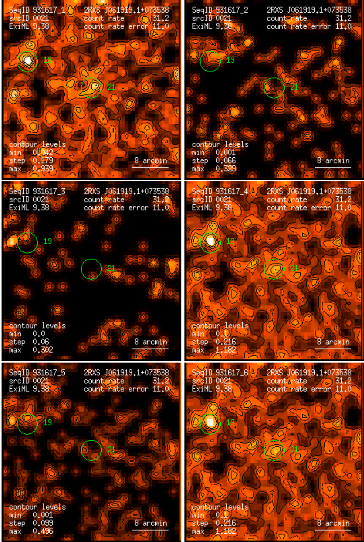
Figure 21: RASS 931617: detection 0021: band rate images, Gaussian filter: (1) PSPC channels 11 – 41, (2) 52 – 90, (3) 91 – 201, (4) 11 – 235, (5) 52 – 201, (6) 11 – 201. Broad band rates in counts/ks. Band rate contour levels in counts/ks/arcmin 2 .
