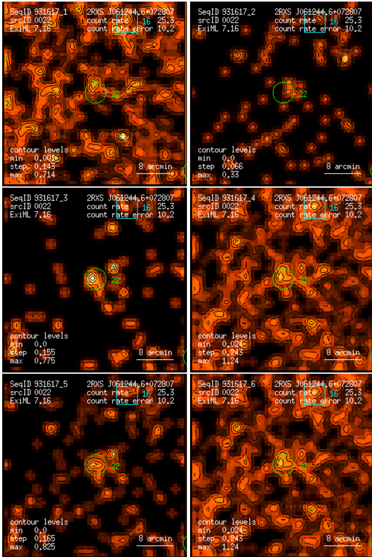
Figure 22: RASS 931617: detection 0022: band rate images, Gaussian filter: (1) PSPC channels 11 – 41, (2) 52 – 90, (3) 91 – 201, (4) 11 – 235, (5) 52 – 201, (6) 11 – 201. Broad band rates in counts/ks. Band rate contour levels in counts/ks/arcmin 2 .
