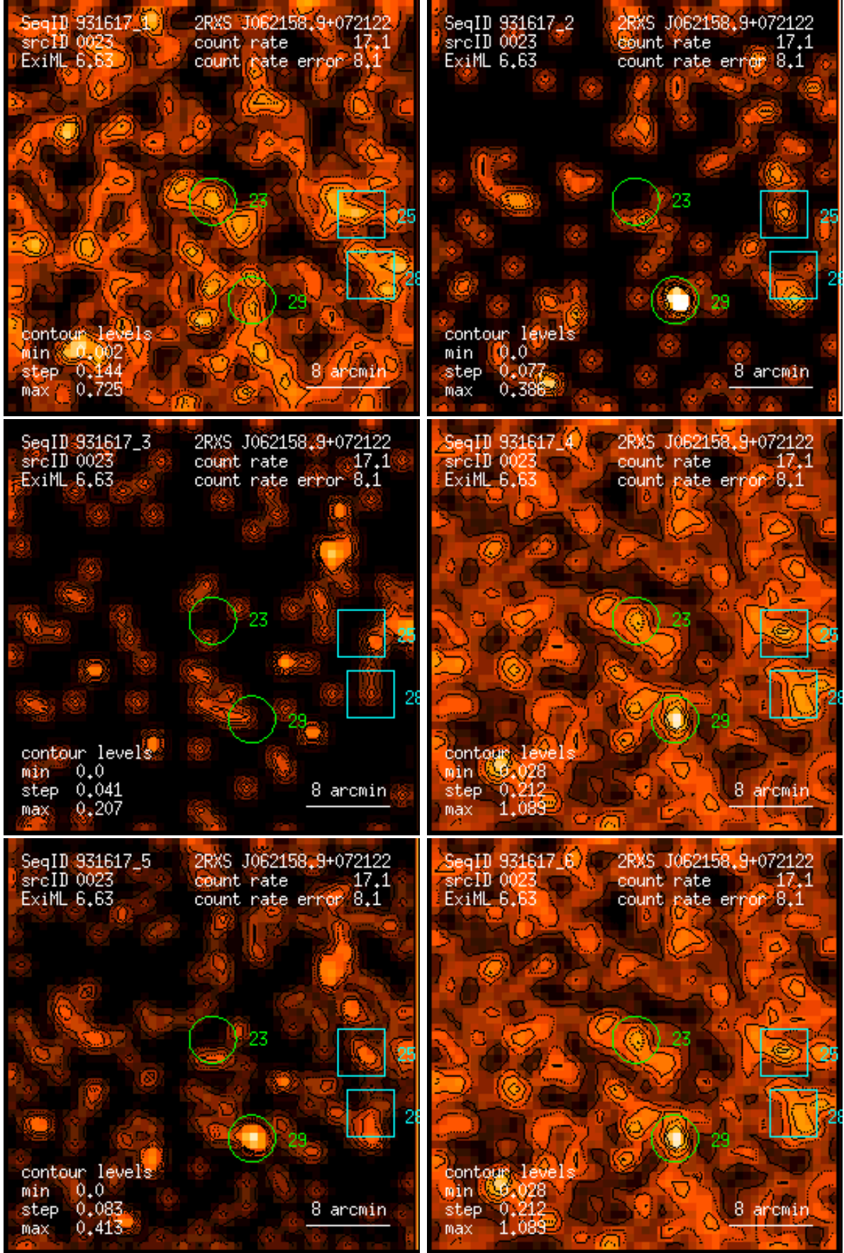
Figure 23: RASS 931617: detection 0023: band rate images, Gaussian filter: (1) PSPC channels 11 – 41, (2) 52 – 90, (3) 91 – 201, (4) 11 – 235, (5) 52 – 201, (6) 11 – 201. Broad band rates in counts/ks. Band rate contour levels in counts/ks/arcmin 2 .
