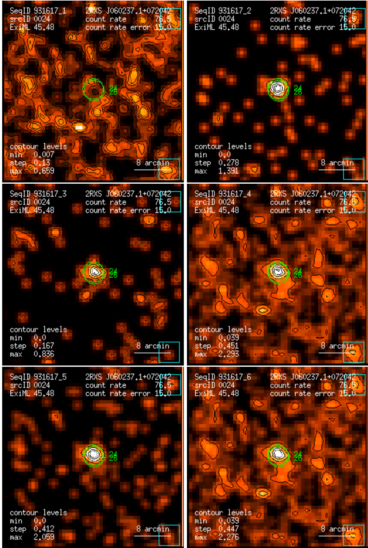
Figure 24: RASS 931617: detection 0024: band rate images, Gaussian filter: (1) PSPC channels 11 – 41, (2) 52 – 90, (3) 91 – 201, (4) 11 – 235, (5) 52 – 201, (6) 11 – 201. Broad band rates in counts/ks. Band rate contour levels in counts/ks/arcmin 2 .
