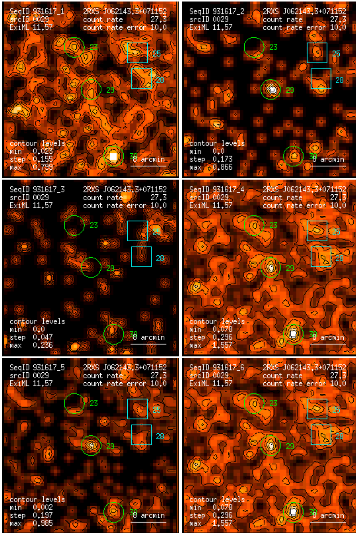
Figure 29: RASS 931617: detection 0029: band rate images, Gaussian filter: (1) PSPC channels 11 – 41, (2) 52 – 90, (3) 91 – 201, (4) 11 – 235, (5) 52 – 201, (6) 11 – 201. Broad band rates in counts/ks. Band rate contour levels in counts/ks/arcmin 2 .
