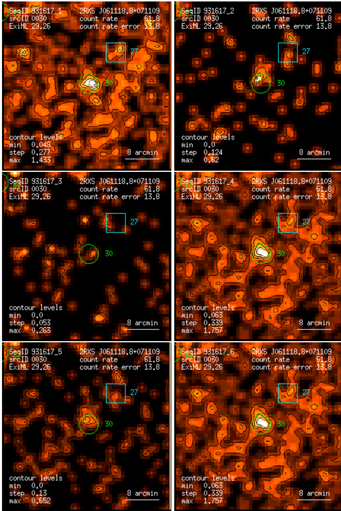
Figure 30: RASS 931617: detection 0030: band rate images, Gaussian filter: (1) PSPC channels 11 – 41, (2) 52 – 90, (3) 91 – 201, (4) 11 – 235, (5) 52 – 201, (6) 11 – 201. Broad band rates in counts/ks. Band rate contour levels in counts/ks/arcmin 2 .
