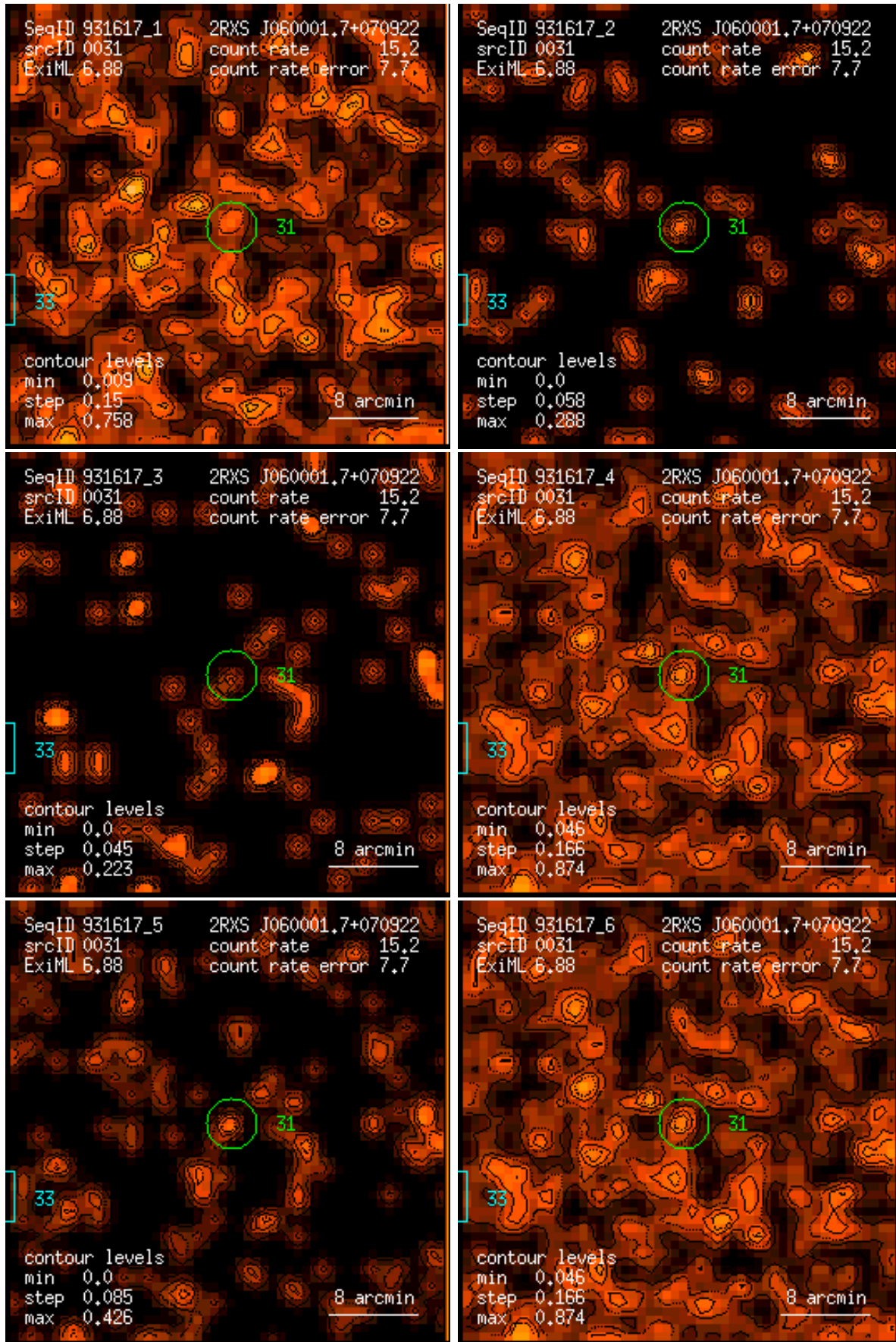
Figure 31: RASS 931617: detection 0031: band rate images, Gaussian filter: (1) PSPC channels 11 – 41, (2) 52 – 90, (3) 91 – 201, (4) 11 – 235, (5) 52 – 201, (6) 11 – 201. Broad band rates in counts/ks. Band rate contour levels in counts/ks/arcmin 2 .
