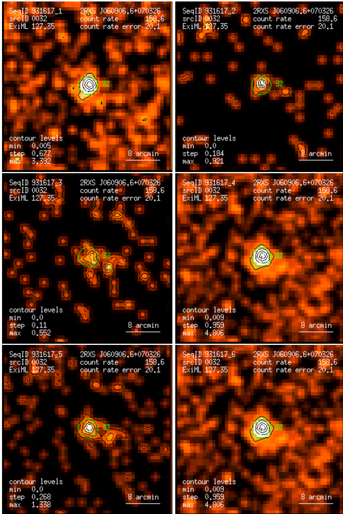
Figure 32: RASS 931617: detection 0032: band rate images, Gaussian filter: (1) PSPC channels 11 – 41, (2) 52 – 90, (3) 91 – 201, (4) 11 – 235, (5) 52 – 201, (6) 11 – 201. Broad band rates in counts/ks. Band rate contour levels in counts/ks/arcmin 2 .
