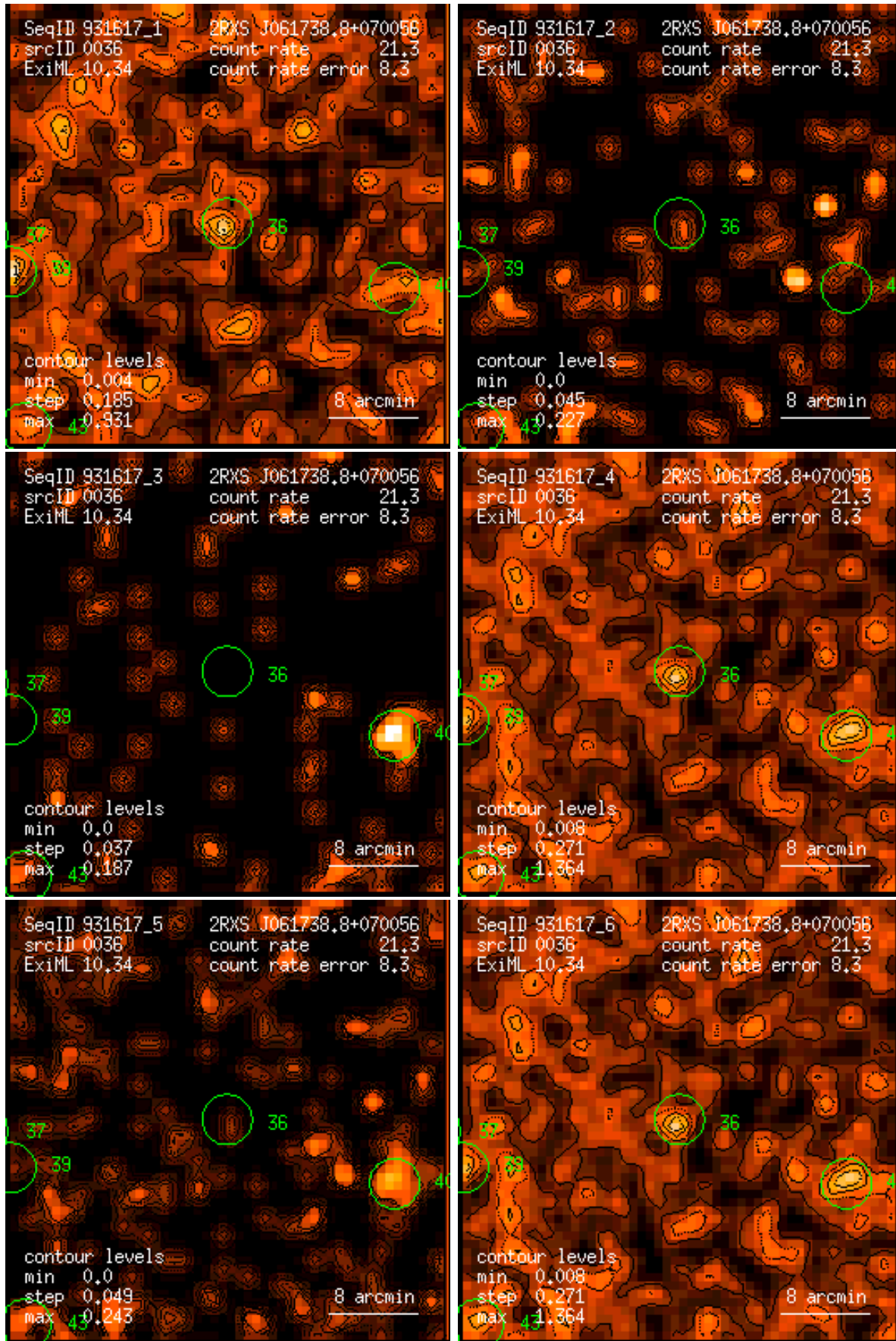
Figure 36: RASS 931617: detection 0036: band rate images, Gaussian filter: (1) PSPC channels 11 – 41, (2) 52 – 90, (3) 91 – 201, (4) 11 – 235, (5) 52 – 201, (6) 11 – 201. Broad band rates in counts/ks. Band rate contour levels in counts/ks/arcmin 2 .
