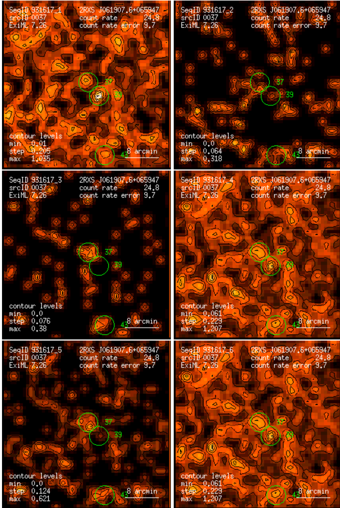
Figure 37: RASS 931617: detection 0037: band rate images, Gaussian filter: (1) PSPC channels 11 – 41, (2) 52 – 90, (3) 91 – 201, (4) 11 – 235, (5) 52 – 201, (6) 11 – 201. Broad band rates in counts/ks. Band rate contour levels in counts/ks/arcmin 2 .
