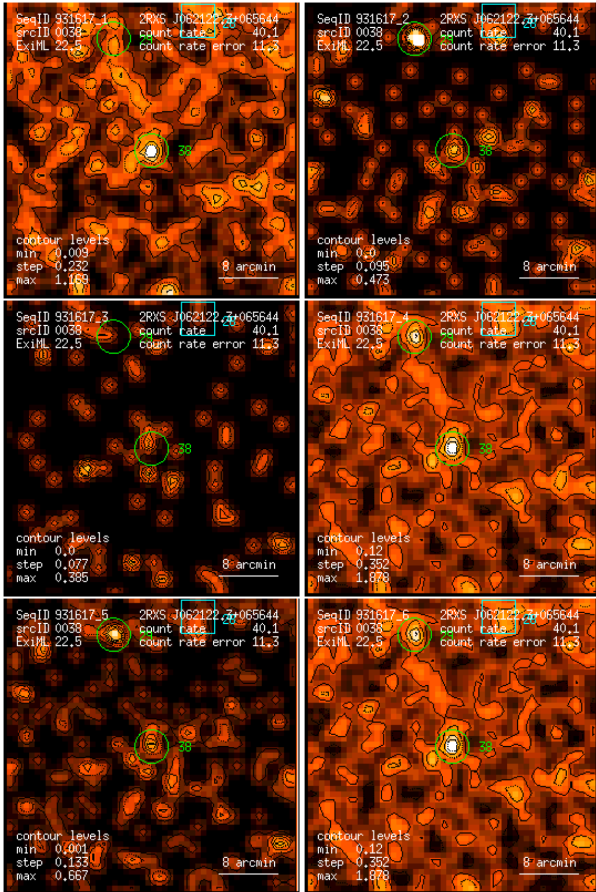
Figure 38: RASS 931617: detection 0038: band rate images, Gaussian filter: (1) PSPC channels 11 – 41, (2) 52 – 90, (3) 91 – 201, (4) 11 – 235, (5) 52 – 201, (6) 11 – 201. Broad band rates in counts/ks. Band rate contour levels in counts/ks/arcmin 2 .
