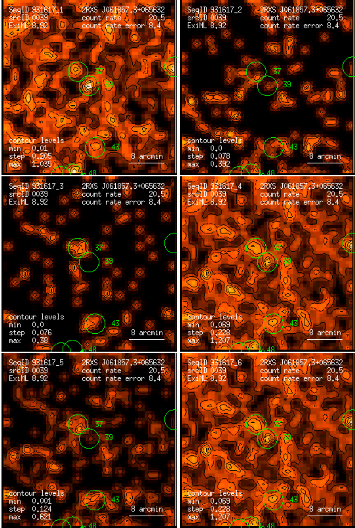
Figure 39: RASS 931617: detection 0039: band rate images, Gaussian filter: (1) PSPC channels 11 – 41, (2) 52 – 90, (3) 91 – 201, (4) 11 – 235, (5) 52 – 201, (6) 11 – 201. Broad band rates in counts/ks. Band rate contour levels in counts/ks/arcmin 2 .
