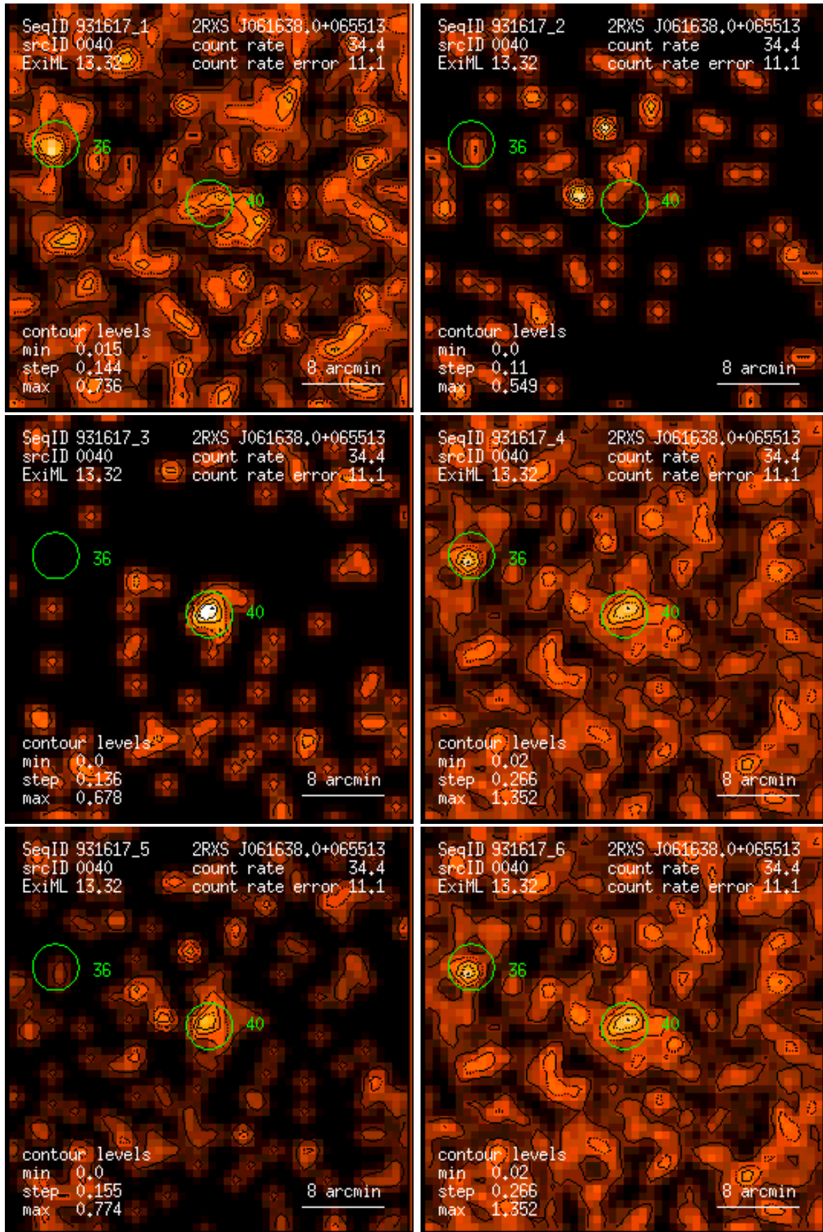
Figure 40: RASS 931617: detection 0040: band rate images, Gaussian filter: (1) PSPC channels 11 – 41, (2) 52 – 90, (3) 91 – 201, (4) 11 – 235, (5) 52 – 201, (6) 11 – 201. Broad band rates in counts/ks. Band rate contour levels in counts/ks/arcmin 2 .
