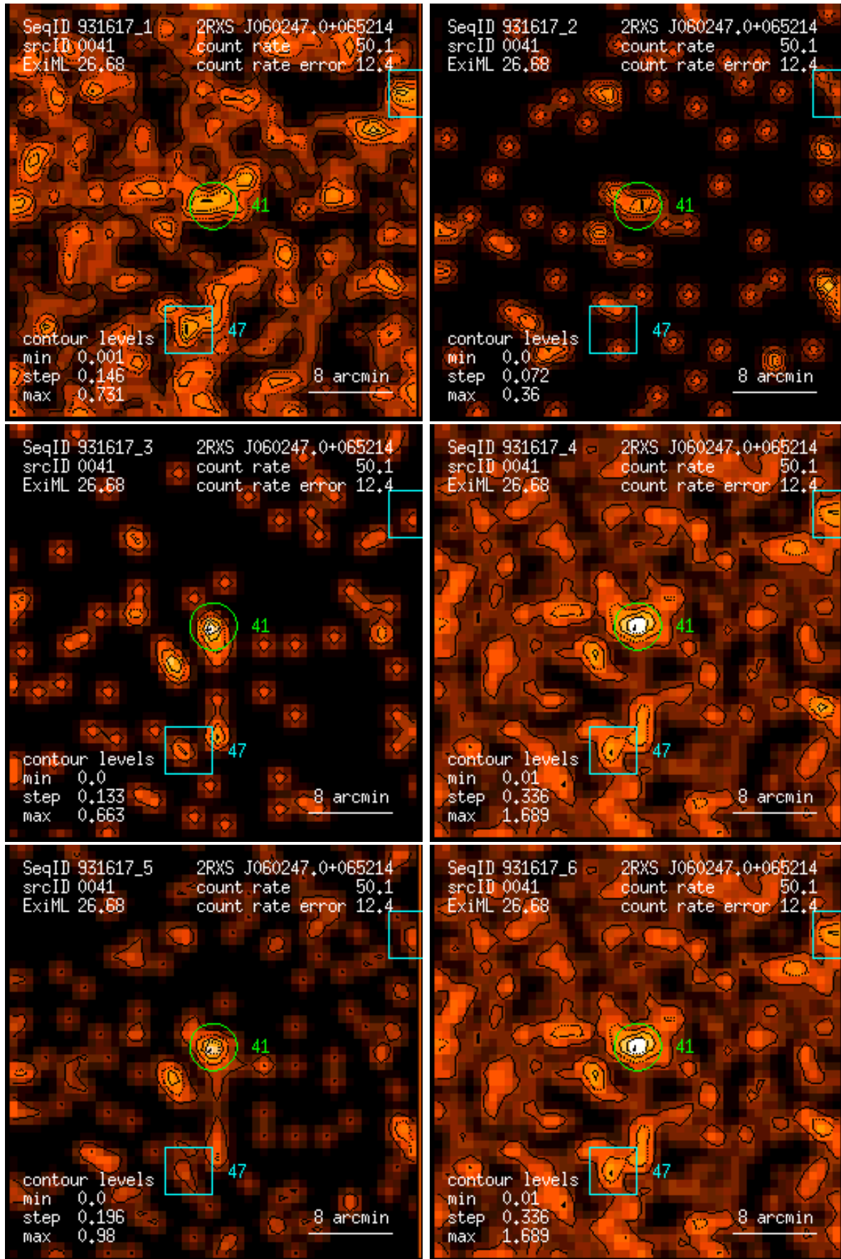
Figure 41: RASS 931617: detection 0041: band rate images, Gaussian filter: (1) PSPP channels 11 – 41, (2) 52 – 90, (3) 91 – 201, (4) 11 – 235, (5) 52 – 201, (6) 11 – 201. Broad band rates in counts/ks. Band rate contour levels in counts/ks/arcmin 2 .
