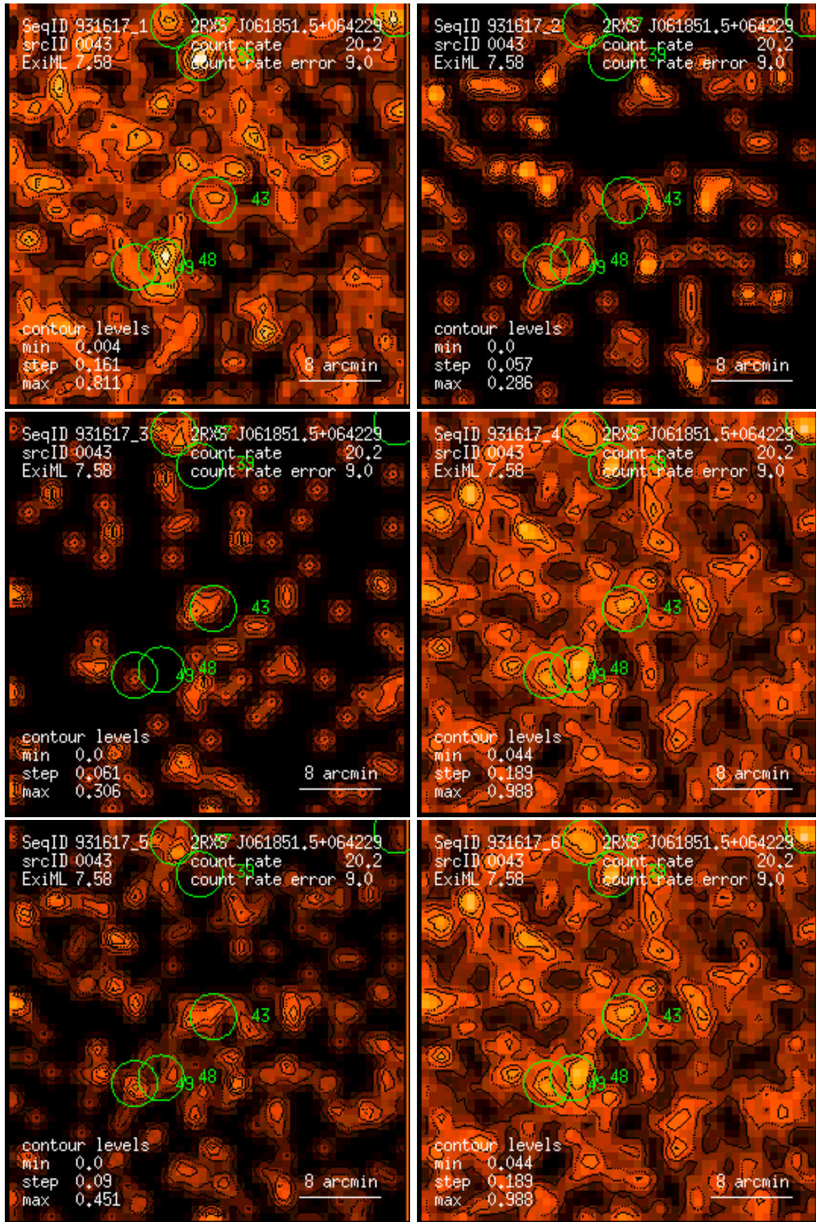
Figure 43: RASS 931617: detection 0043: band rate images, Gaussian filter: (1) PSPC channels 11 – 41, (2) 52 – 90, (3) 91 – 201, (4) 11 – 235, (5) 52 – 201, (6) 11 – 201. Broad band rates in counts/ks. Band rate contour levels in counts/ks/arcmin 2 .
