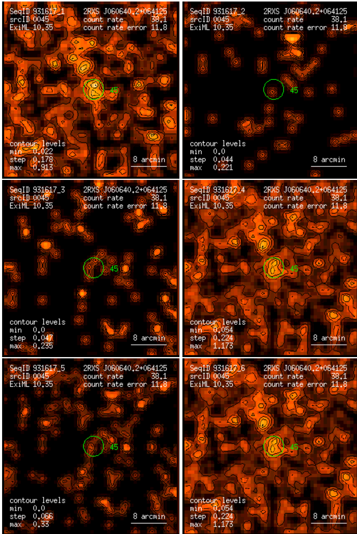
Figure 45: RASS 931617: detection 0045: band rate images, Gaussian filter: (1) PSPC channels 11 – 41, (2) 52 – 90, (3) 91 – 201, (4) 11 – 235, (5) 52 – 201, (6) 11 – 201. Broad band rates in counts/ks. Band rate contour levels in counts/ks/arcmin 2 .
