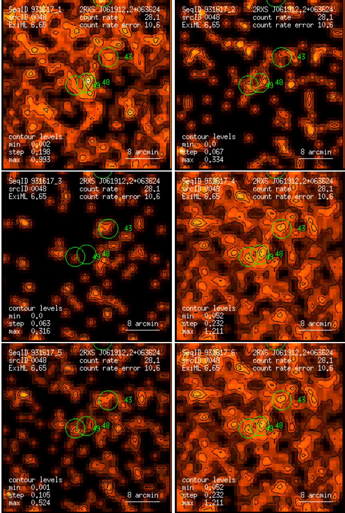
Figure 48: RASS 931617: detection 0048: band rate images, Gaussian filter: (1) PSPC channels 11 – 41, (2) 52 – 90, (3) 91 – 201, (4) 11 – 235, (5) 52 – 201, (6) 11 – 201. Broad band rates in counts/ks. Band rate contour levels in counts/ks/arcmin 2 .
