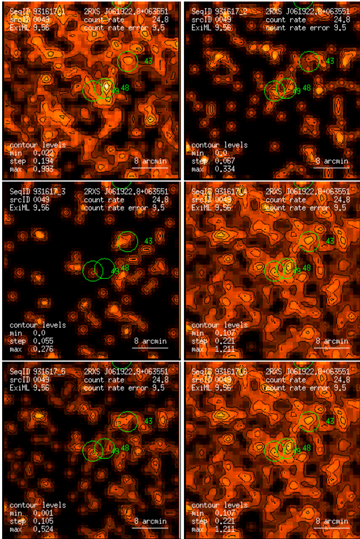
Figure 49: RASS 931617: detection 0049: band rate images, Gaussian filter: (1) PSPC channels 11 – 41, (2) 52 – 90, (3) 91 – 201, (4) 11 – 235, (5) 52 – 201, (6) 11 – 201. Broad band rates in counts/ks. Band rate contour levels in counts/ks/arcmin 2 .
