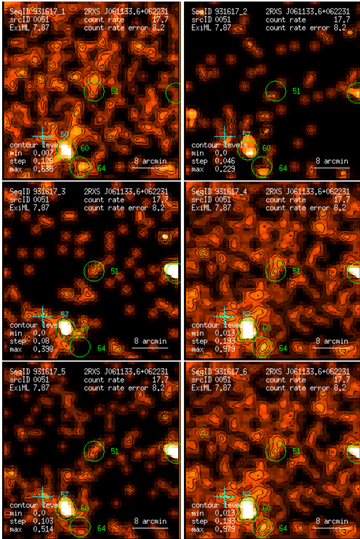
Figure 51: RASS 931617: detection 0051: band rate images, Gaussian filter: (1) PSPC channels 11 – 41, (2) 52 – 90, (3) 91 – 201, (4) 11 – 235, (5) 52 – 201, (6) 11 – 201. Broad band rates in counts/ks. Band rate contour levels in counts/ks/arcmin 2 .
