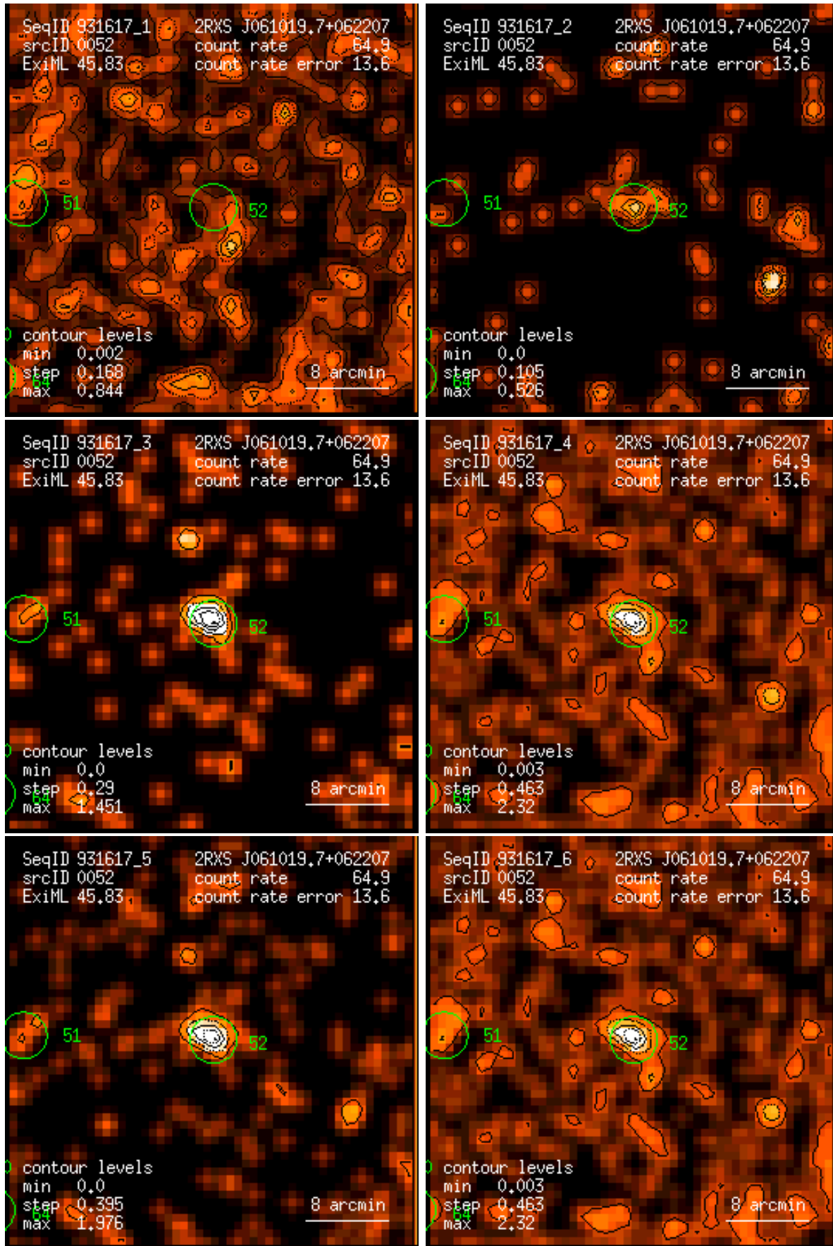
Figure 52: RASS 931617: detection 0052: band rate images, Gaussian filter: (1) PSPC channels 11 – 41, (2) 52 – 90, (3) 91 – 201, (4) 11 – 235, (5) 52 – 201, (6) 11 – 201. Broad band rates in counts/ks. Band rate contour levels in counts/ks/arcmin 2 .
