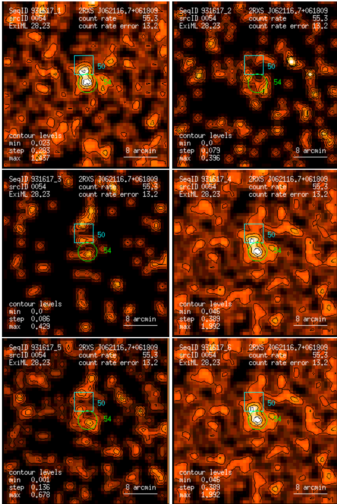
Figure 54: RASS 931617: detection 0054: band rate images, Gaussian filter: (1) PSPC channels 11 – 41, (2) 52 – 90, (3) 91 – 201, (4) 11 – 235, (5) 52 – 201, (6) 11 – 201. Broad band rates in counts/ks. Band rate contour levels in counts/ks/arcmin 2 .
