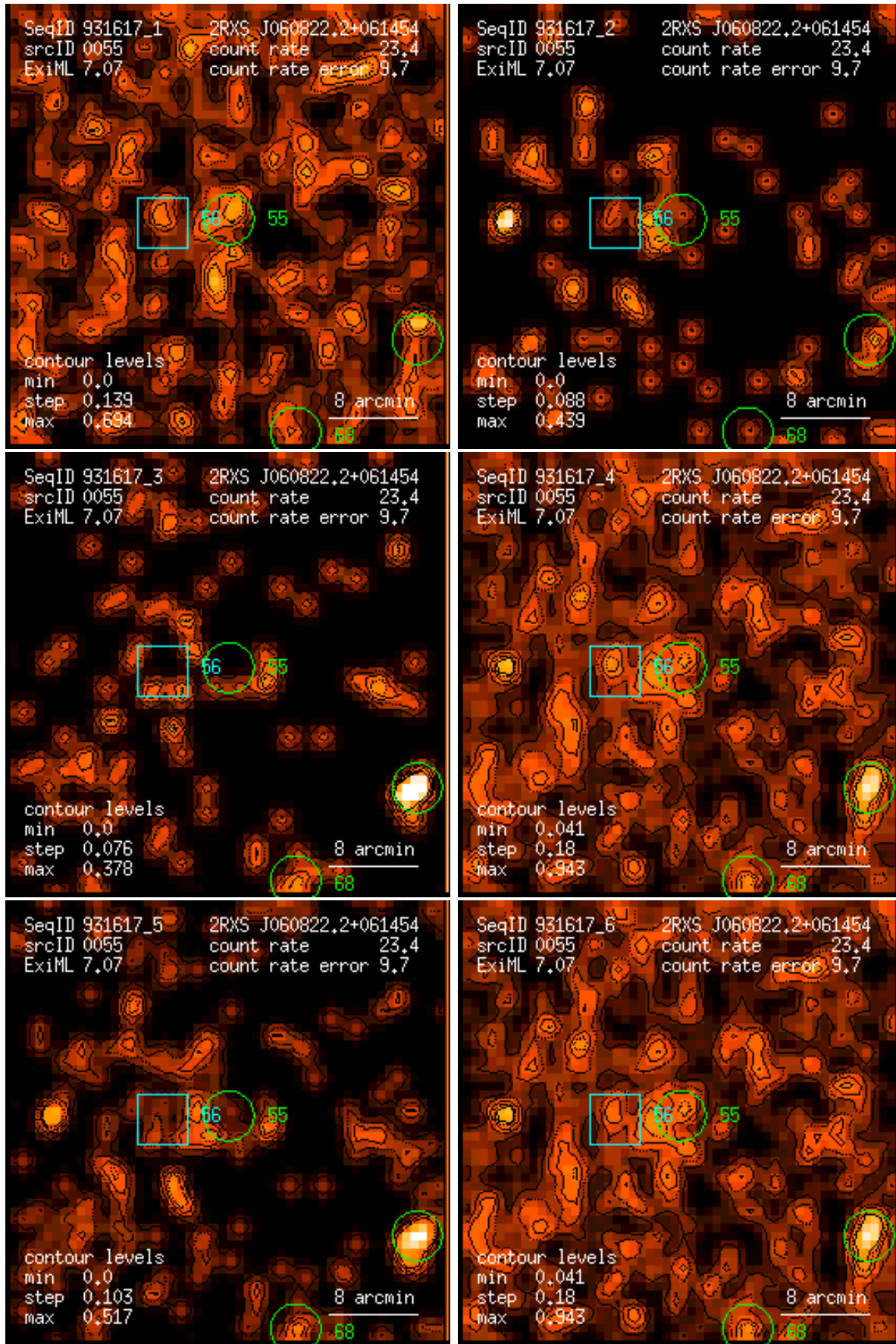
Figure 55: RASS 931617: detection 0055: band rate images, Gaussian filter: (1) PSPC channels 11 – 41, (2) 52 – 90, (3) 91 – 201, (4) 11 – 235, (5) 52 – 201, (6) 11 – 201. Broad band rates in counts/ks. Band rate contour levels in counts/ks/arcmin 2 .
