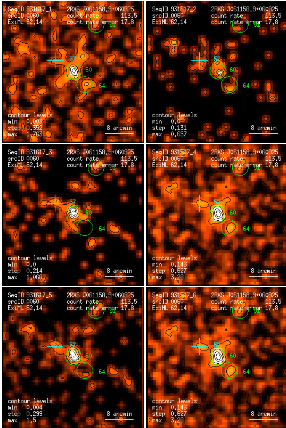
Figure 60: RASS 931617: detection 0060: band rate images, Gaussian filter: (1) PSPC channels 11 – 41, (2) 52 – 90, (3) 91 – 201, (4) 11 – 235, (5) 52 – 201, (6) 11 – 201. Broad band rates in counts/ks. Band rate contour levels in counts/ks/arcmin 2 .
