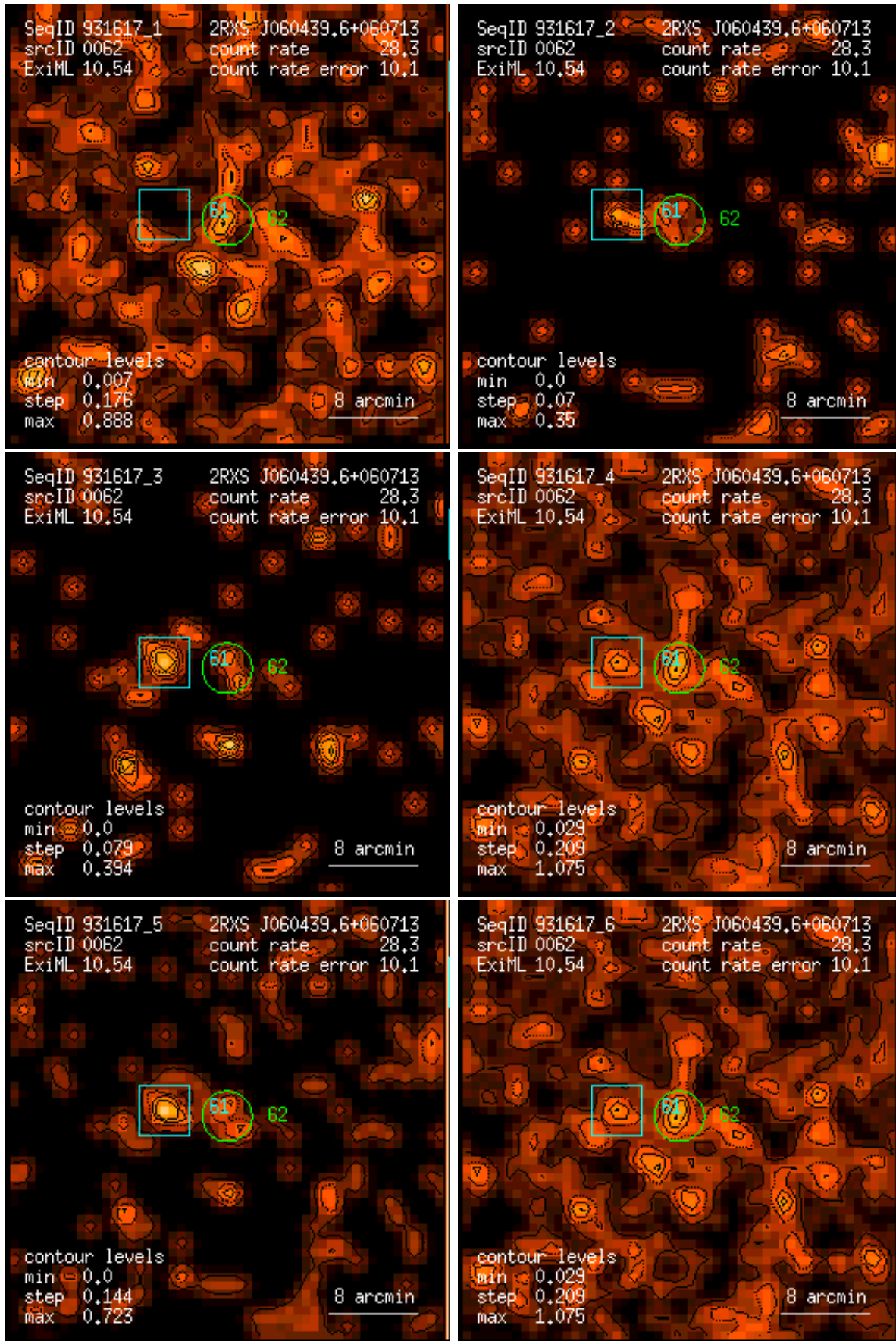
Figure 62: RASS 931617: detection 0062: band rate images, Gaussian filter: (1) PSPC channels 11 – 41, (2) 52 – 90, (3) 91 – 201, (4) 11 – 235, (5) 52 – 201, (6) 11 – 201. Broad band rates in counts/ks. Band rate contour levels in counts/ks/arcmin 2 .
