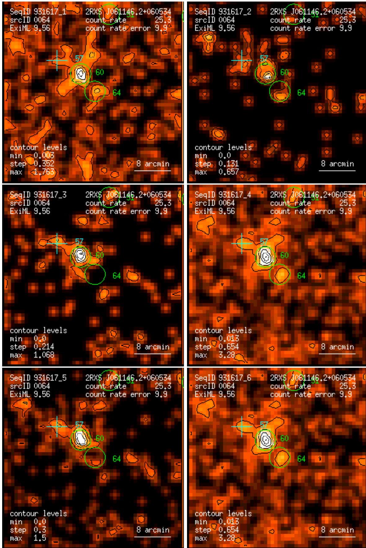
Figure 64: RASS 931617: detection 0064: band rate images, Gaussian filter: (1) PSPC channels 11 – 41, (2) 52 – 90, (3) 91 – 201, (4) 11 – 235, (5) 52 – 201, (6) 11 – 201. Broad band rates in counts/ks. Band rate contour levels in counts/ks/arcmin 2 .
