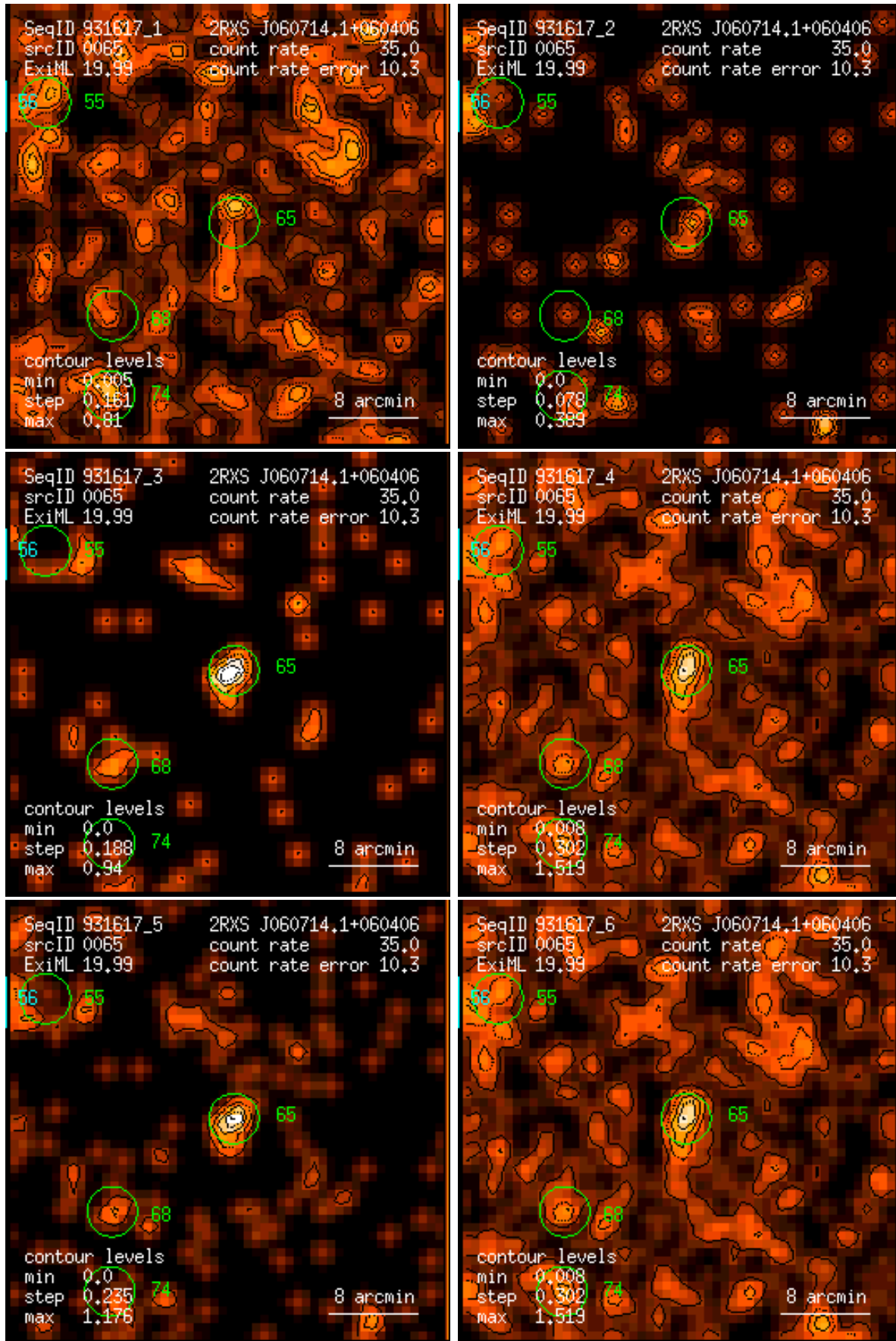
Figure 65: RASS 931617: detection 0065: band rate images, Gaussian filter: (1) PSPC channels 11 – 41, (2) 52 – 90, (3) 91 – 201, (4) 11 – 235, (5) 52 – 201, (6) 11 – 201. Broad band rates in counts/ks. Band rate contour levels in counts/ks/arcmin 2 .
