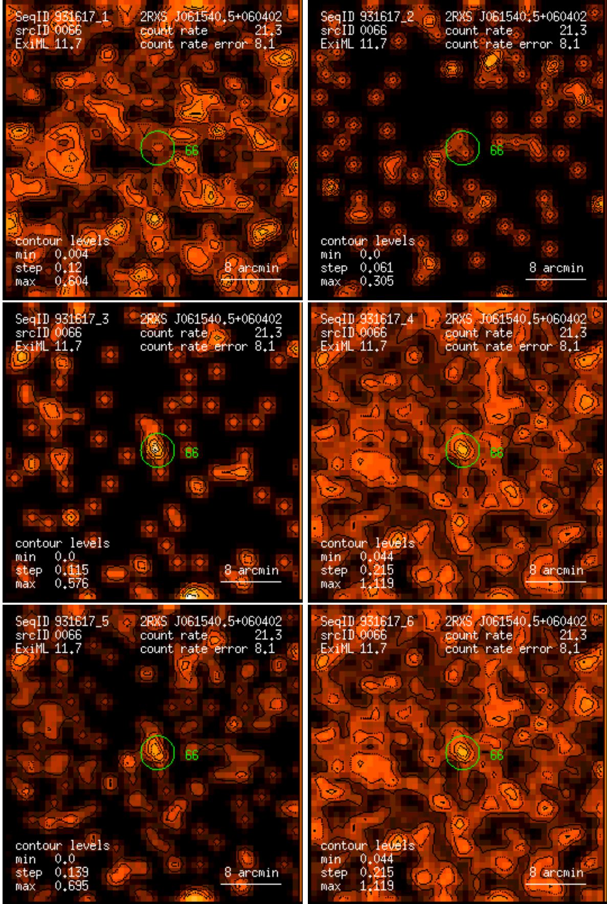
Figure 66: RASS 931617: detection 0066: band rate images, Gaussian filter: (1) PSPC channels 11 – 41, (2) 52 – 90, (3) 91 – 201, (4) 11 – 235, (5) 52 – 201, (6) 11 – 201. Broad band rates in counts/ks. Band rate contour levels in counts/ks/arcmin 2 .
