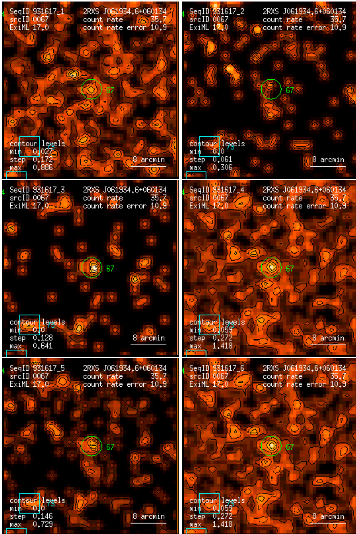
Figure 67: RASS 931617: detection 0067: band rate images, Gaussian filter: (1) PSPC channels 11 – 41, (2) 52 – 90, (3) 91 – 201, (4) 11 – 235, (5) 52 – 201, (6) 11 – 201. Broad band rates in counts/ks. Band rate contour levels in counts/ks/arcmin 2 .
