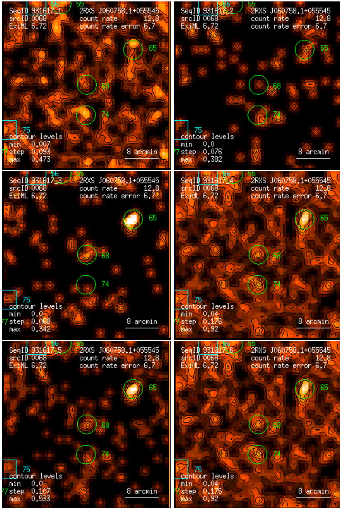
Figure 68: RASS 931617: detection 0068: band rate images, Gaussian filter: (1) PSPC channels 11 – 41, (2) 52 – 90, (3) 91 – 201, (4) 11 – 235, (5) 52 – 201, (6) 11 – 201. Broad band rates in counts/ks. Band rate contour levels in counts/ks/arcmin 2 .
