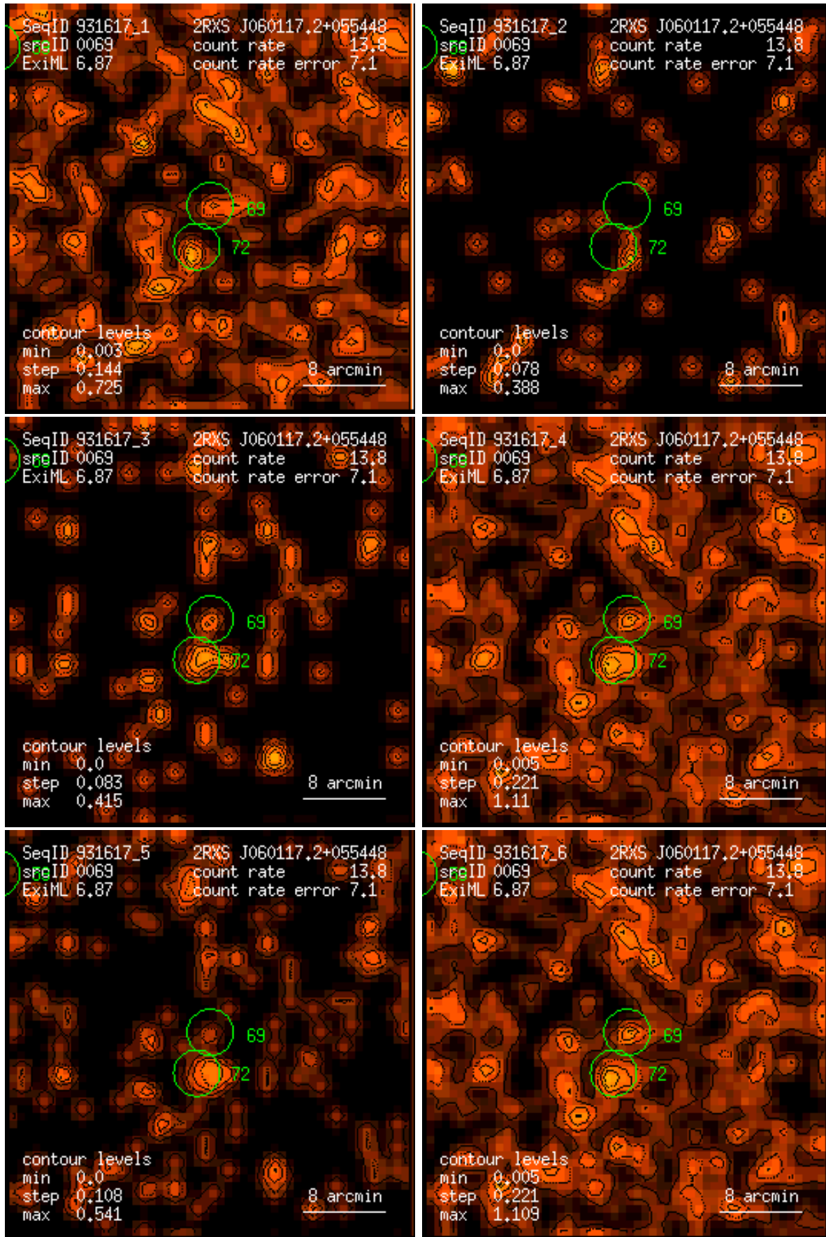
Figure 69: RASS 931617: detection 0069: band rate images, Gaussian filter: (1) PSPC channels 11 – 41, (2) 52 – 90, (3) 91 – 201, (4) 11 – 235, (5) 52 – 201, (6) 11 – 201. Broad band rates in counts/ks. Band rate contour levels in counts/ks/arcmin 2 .
