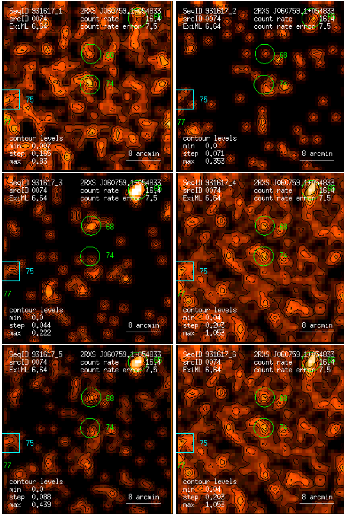
Figure 74: RASS 931617: detection 0074: band rate images, Gaussian filter: (1) PSPC channels 11 – 41, (2) 52 – 90, (3) 91 – 201, (4) 11 – 235, (5) 52 – 201, (6) 11 – 201. Broad band rates in counts/ks. Band rate contour levels in counts/ks/arcmin 2 .
