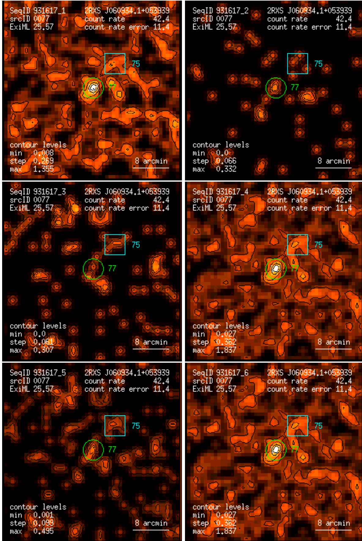
Figure 77: RASS 931617: detection 0077: band rate images, Gaussian filter: (1) PSPC channels 11 – 41, (2) 52 – 90, (3) 91 – 201, (4) 11 – 235, (5) 52 – 201, (6) 11 – 201. Broad band rates in counts/ks. Band rate contour levels in counts/ks/arcmin 2 .
