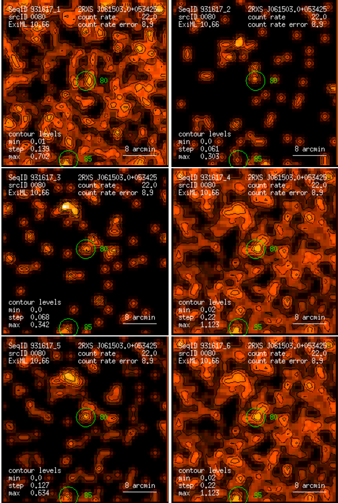
Figure 80: RASS 931617: detection 0080: band rate images, Gaussian filter: (1) PSPC channels 11 – 41, (2) 52 – 90, (3) 91 – 201, (4) 11 – 235, (5) 52 – 201, (6) 11 – 201. Broad band rates in counts/ks. Band rate contour levels in counts/ks/arcmin 2 .
