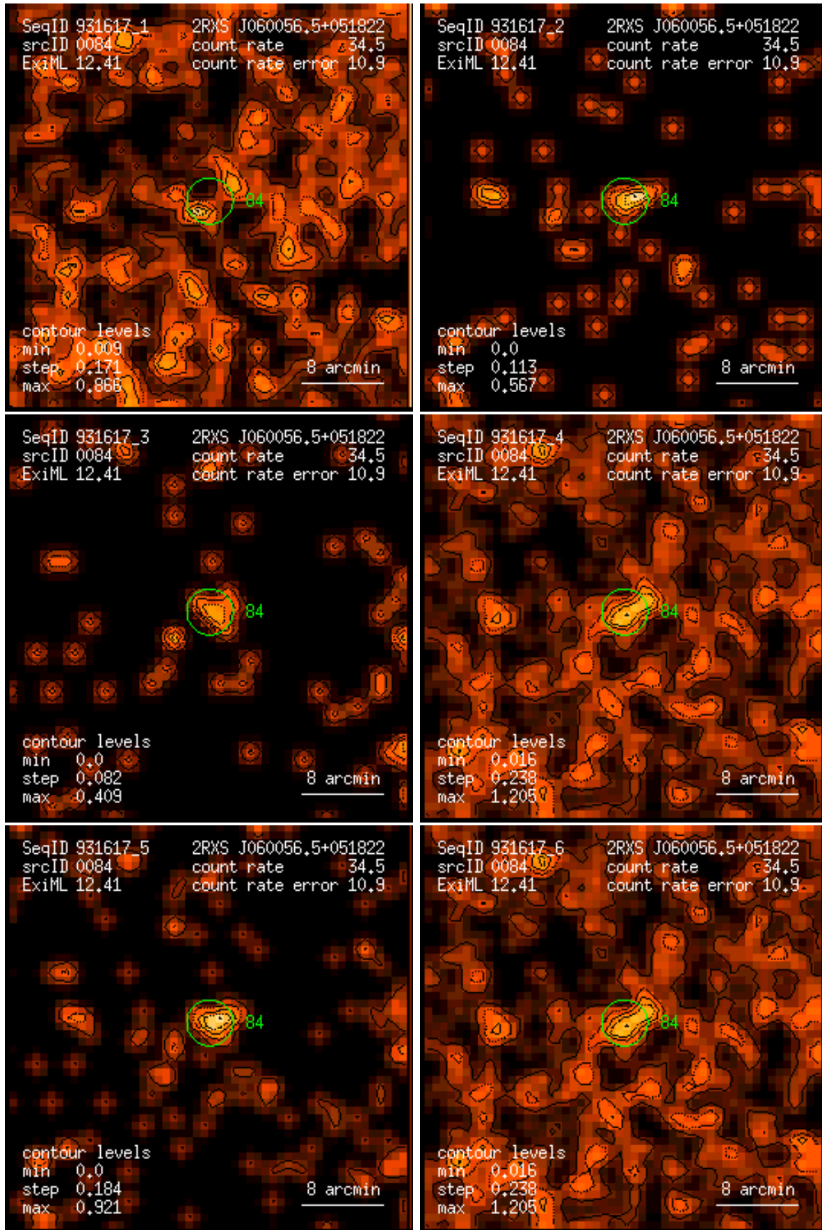
Figure 84: RASS 931617: detection 0084: band rate images, Gaussian filter: (1) PSPC channels 11 – 41, (2) 52 – 90, (3) 91 – 201, (4) 11 – 235, (5) 52 – 201, (6) 11 – 201. Broad band rates in counts/ks. Band rate contour levels in counts/ks/arcmin 2 .
