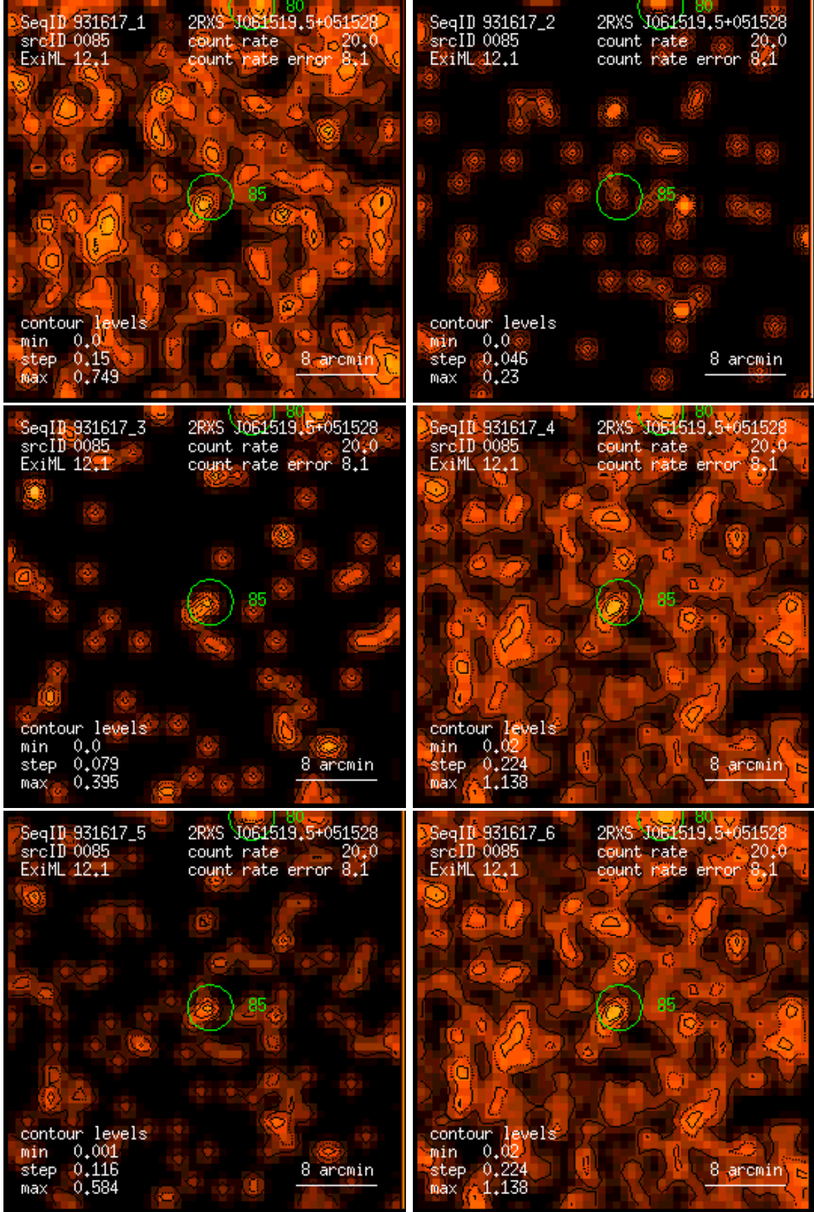
Figure 85: RASS 931617: detection 0085: band rate images, Gaussian filter: (1) PSPC channels 11 – 41, (2) 52 – 90, (3) 91 – 201, (4) 11 – 235, (5) 52 – 201, (6) 11 – 201. Broad band rates in counts/ks. Band rate contour levels in counts/ks/arcmin 2 .
