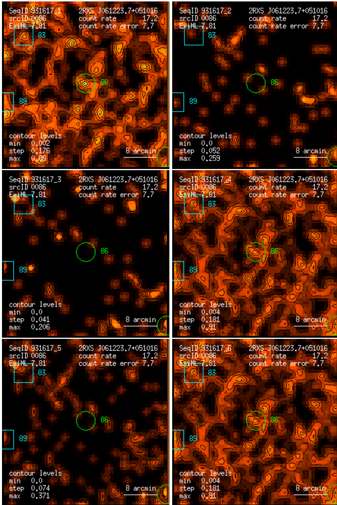
Figure 86: RASS 931617: detection 0086: band rate images, Gaussian filter: (1) PSPC channels 11 – 41, (2) 52 – 90, (3) 91 – 201, (4) 11 – 235, (5) 52 – 201, (6) 11 – 201. Broad band rates in counts/ks. Band rate contour levels in counts/ks/arcmin 2 .
