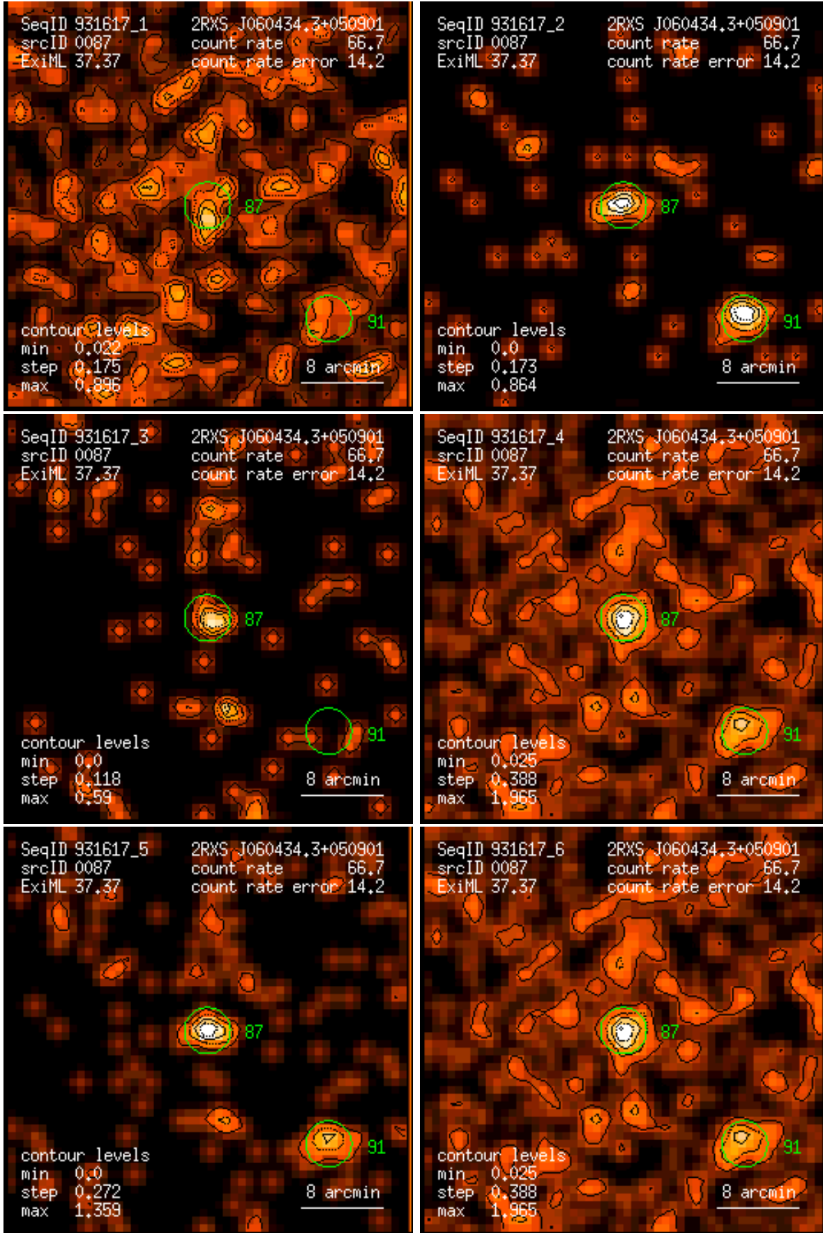
Figure 87: RASS 931617: detection 0087: band rate images, Gaussian filter: (1) PSPC channels 11 – 41, (2) 52 – 90, (3) 91 – 201, (4) 11 – 235, (5) 52 – 201, (6) 11 – 201. Broad band rates in counts/ks. Band rate contour levels in counts/ks/arcmin 2 .
