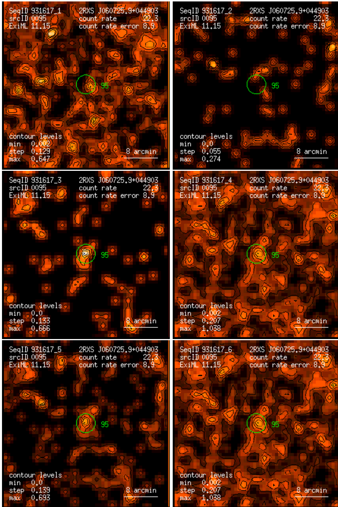
Figure 95: RASS 931617: detection 0095: band rate images, Gaussian filter: (1) PSPC channels 11 – 41, (2) 52 – 90, (3) 91 – 201, (4) 11 – 235, (5) 52 – 201, (6) 11 – 201. Broad band rates in counts/ks. Band rate contour levels in counts/ks/arcmin 2 .
