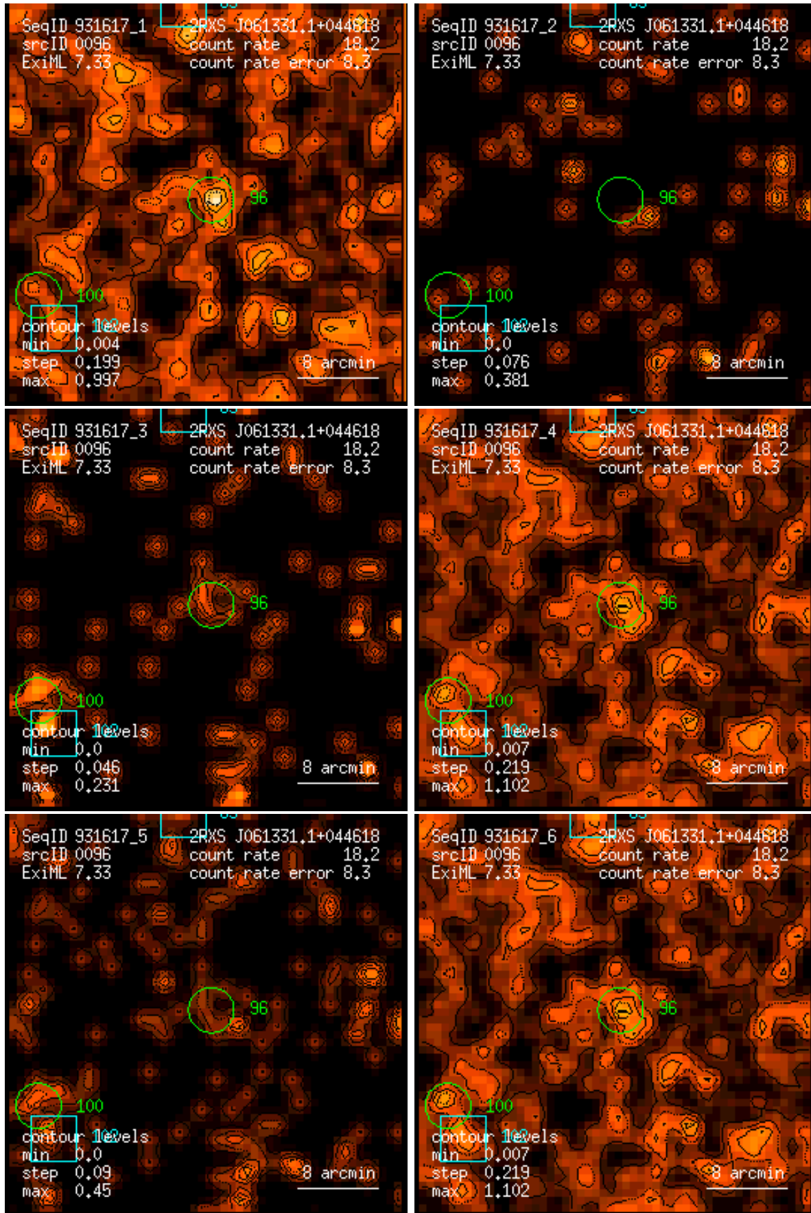
Figure 96: RASS 931617: detection 0096: band rate images, Gaussian filter: (1) PSPC channels 11 – 41, (2) 52 – 90, (3) 91 – 201, (4) 11 – 235, (5) 52 – 201, (6) 11 – 201. Broad band rates in counts/ks. Band rate contour levels in counts/ks/arcmin 2 .
