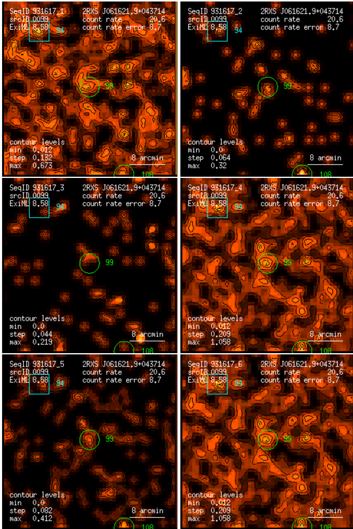
Figure 99: RASS 931617: detection 0099: band rate images, Gaussian filter: (1) PSPC channels 11 – 41, (2) 52 – 90, (3) 91 – 201, (4) 11 – 235, (5) 52 – 201, (6) 11 – 201. Broad band rates in counts/ks. Band rate contour levels in counts/ks/arcmin 2 .
