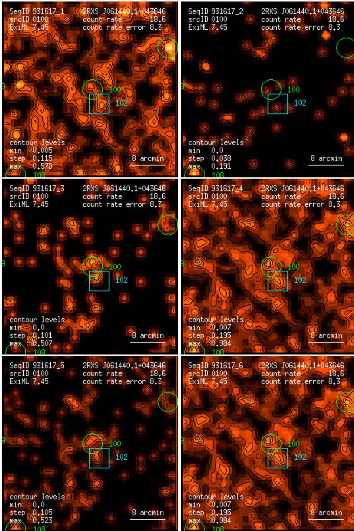
Figure 100: RASS 931617: detection 0100: band rate images, Gaussian filter: (1) PSPC channels 11 – 41, (2) 52 – 90, (3) 91 – 201, (4) 11 – 235, (5) 52 – 201, (6) 11 – 201. Broad band rates in counts/ks. Band rate contour levels in counts/ks/arcmin 2 .
