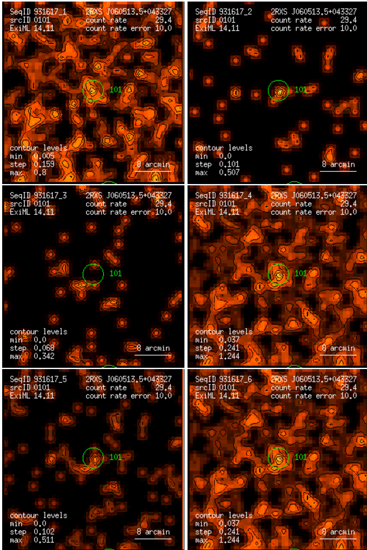
Figure 101: RASS 931617: detection 0101: band rate images, Gaussian filter: (1) PSPC channels 11 – 41, (2) 52 – 90, (3) 91 – 201, (4) 11 – 235, (5) 52 – 201, (6) 11 – 201. Broad band rates in counts/ks. Band rate contour levels in counts/ks/arcmin 2 .
