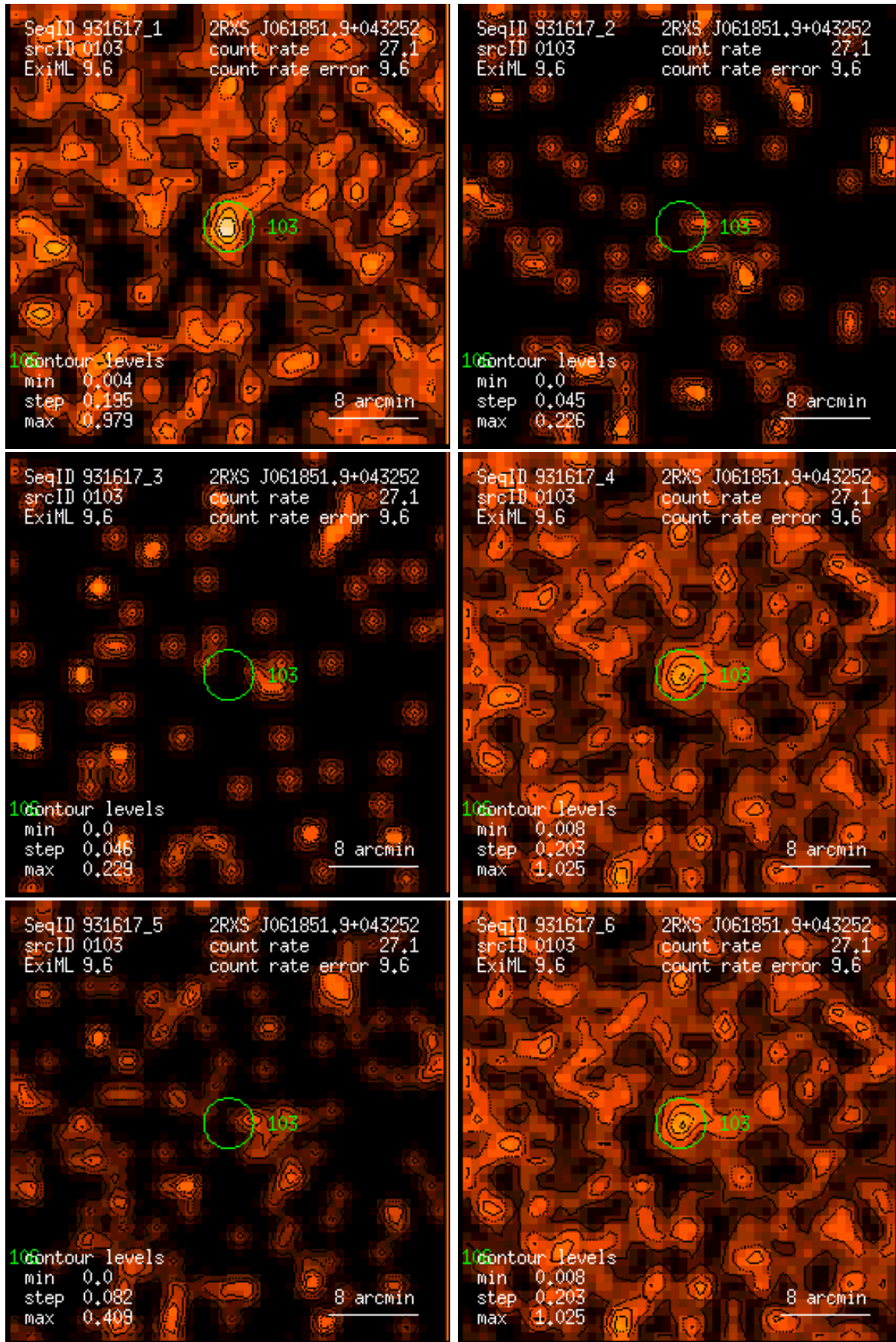
Figure 103: RASS 931617: detection 0103: band rate images, Gaussian filter: (1) PSPC channels 11 – 41, (2) 52 – 90, (3) 91 – 201, (4) 11 – 235, (5) 52 – 201, (6) 11 – 201. Broad band rates in counts/ks. Band rate contour levels in counts/ks/arcmin 2 .
