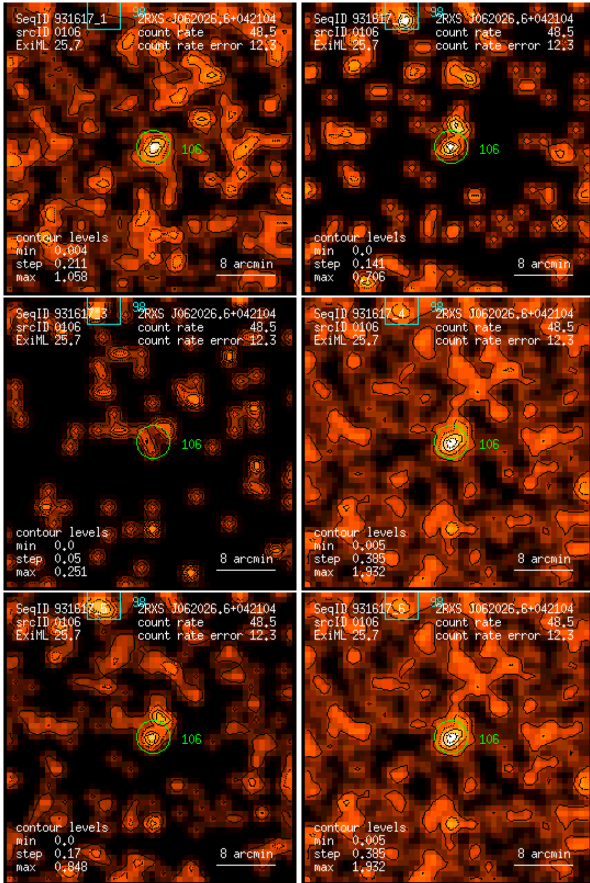
Figure 106: RASS 931617: detection 0106: band rate images, Gaussian filter: (1) PSPC channels 11 – 41, (2) 52 – 90, (3) 91 – 201, (4) 11 – 235, (5) 52 – 201, (6) 11 – 201. Broad band rates in counts/ks. Band rate contour levels in counts/ks/arcmin 2 .
