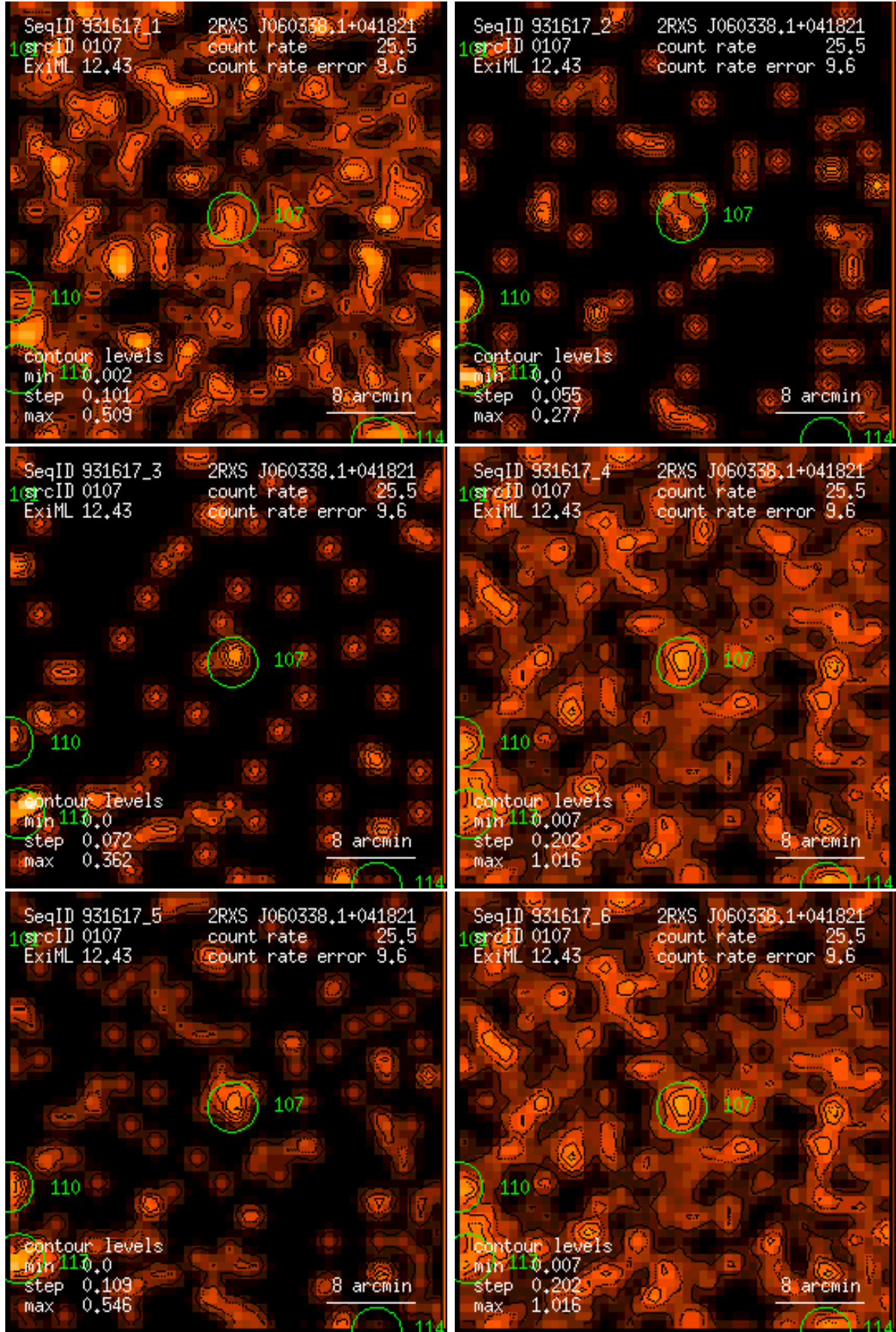
Figure 107: RASS 931617: detection 0107: band rate images, Gaussian filter: (1) PSPC channels 11 – 41, (2) 52 – 90, (3) 91 – 201, (4) 11 – 235, (5) 52 – 201, (6) 11 – 201. Broad band rates in counts/ks. Band rate contour levels in counts/ks/arcmin 2 .
